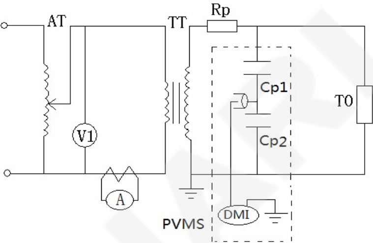
工频试验回路图 (Diagram of power frequency voltage circuit)
